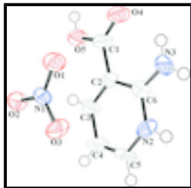
Fig. 1. The structure of the title compound with the atomic labelling scheme. Displacement are drawn at the 50% probability level.
